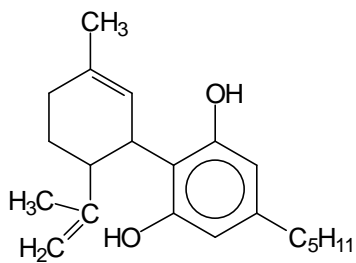
Cannabidiol (CBD)
