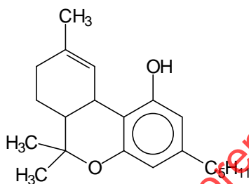
Tetrahydrocannabinol (THC)
