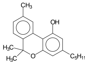
Cannabinol (CBN)
